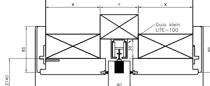
Detalle jamba sup. Escala 1:4
